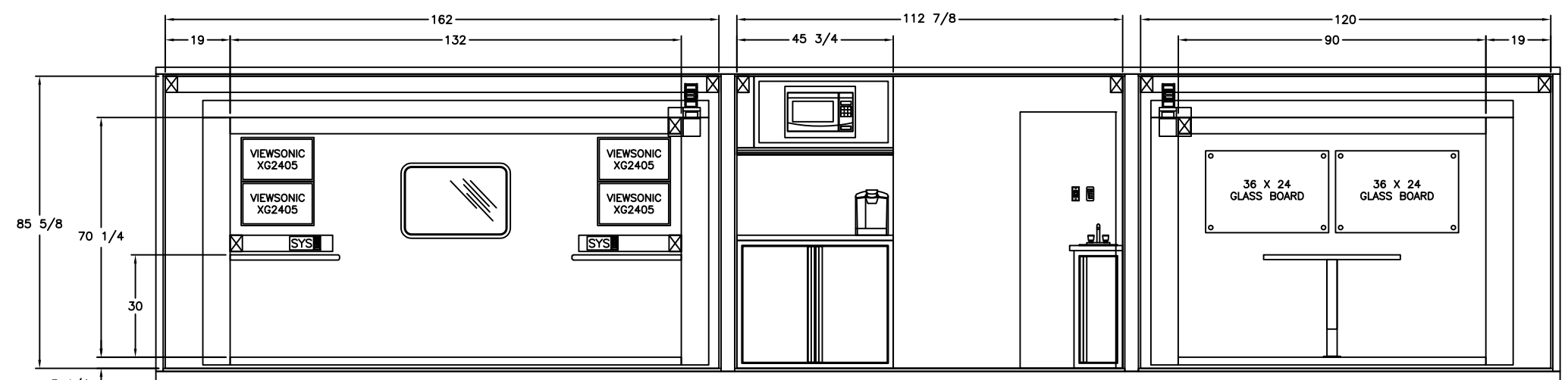
STREET SIDE INTERIOR LAYOUT
