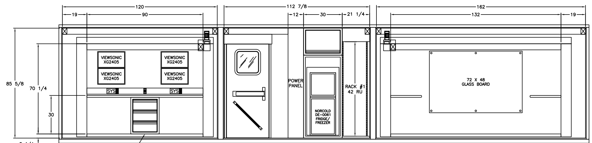
CURB SIDE INTERIOR LAYOUT
