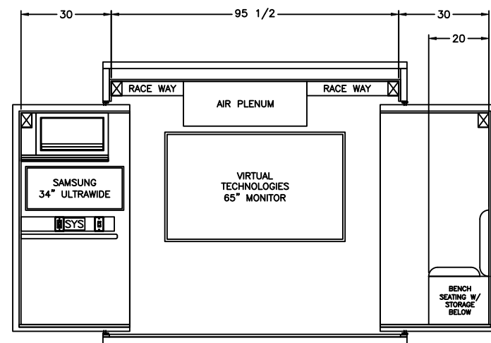
REAR WALL INTERIOR LAYOUT
