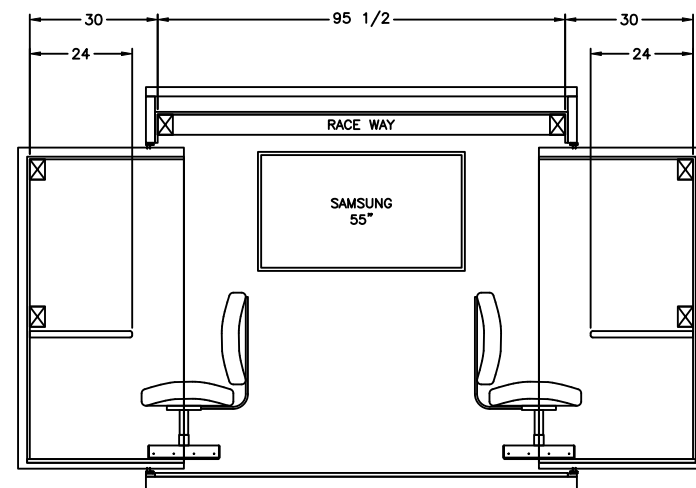
FRONT WALL INTERIOR LAYOUT
