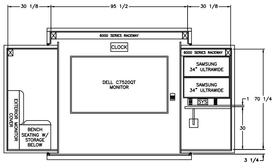
REAR WALL INTERIOR LAYOUT
