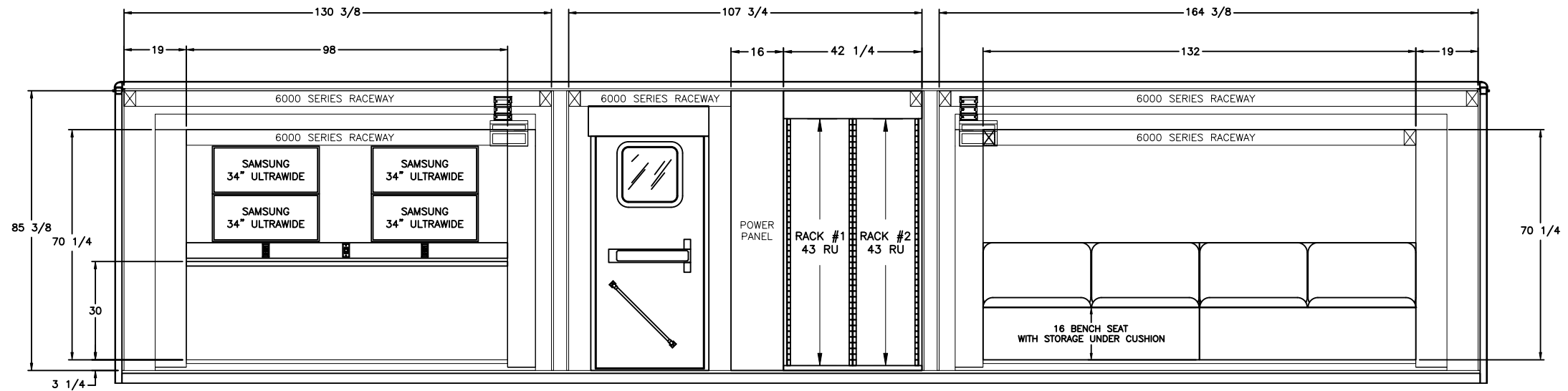
PASSENGERS SIDE INTERIOR LAYOUT
