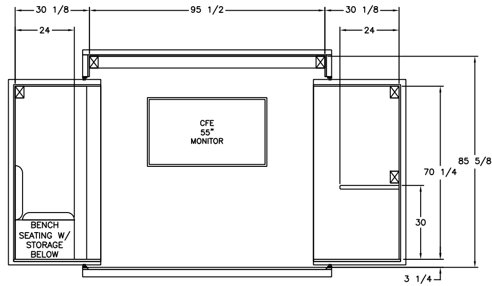
FRONT WALL INTERIOR LAYOUT
