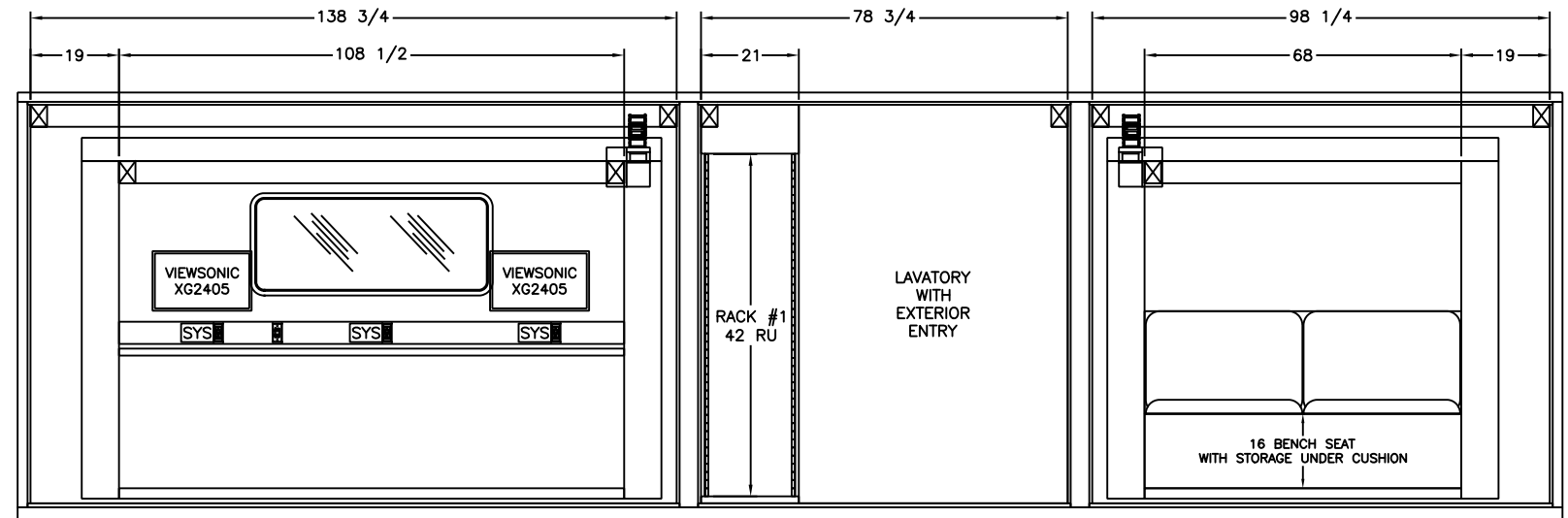
STREET SIDE INTERIOR LAYOUT
