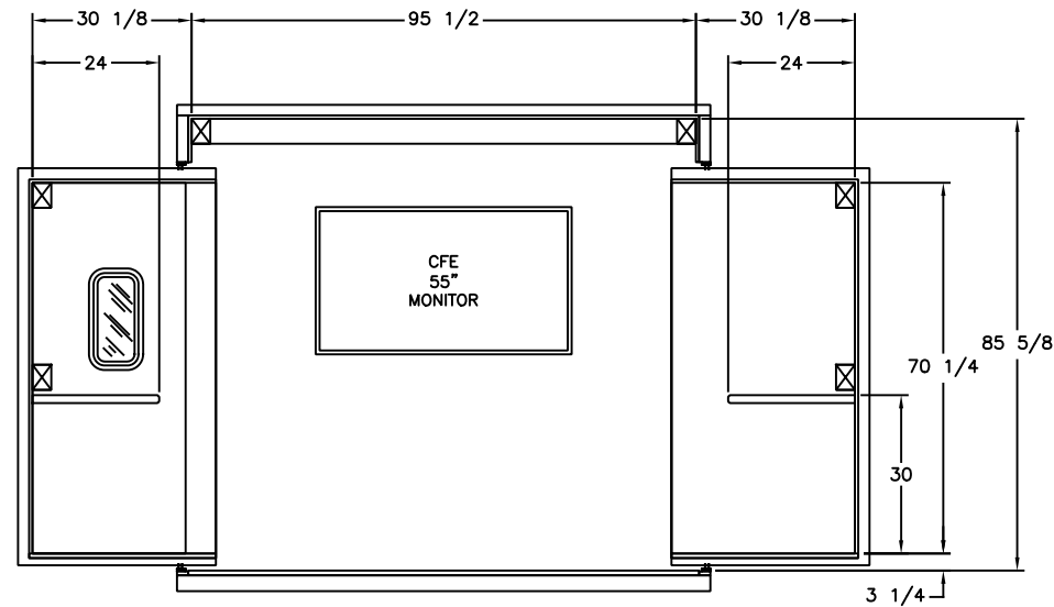
REAR WALL INTERIOR LAYOUT
