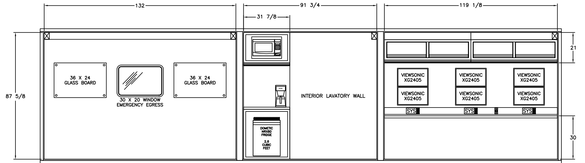
LEFT SIDE INTERIOR LAYOUT
