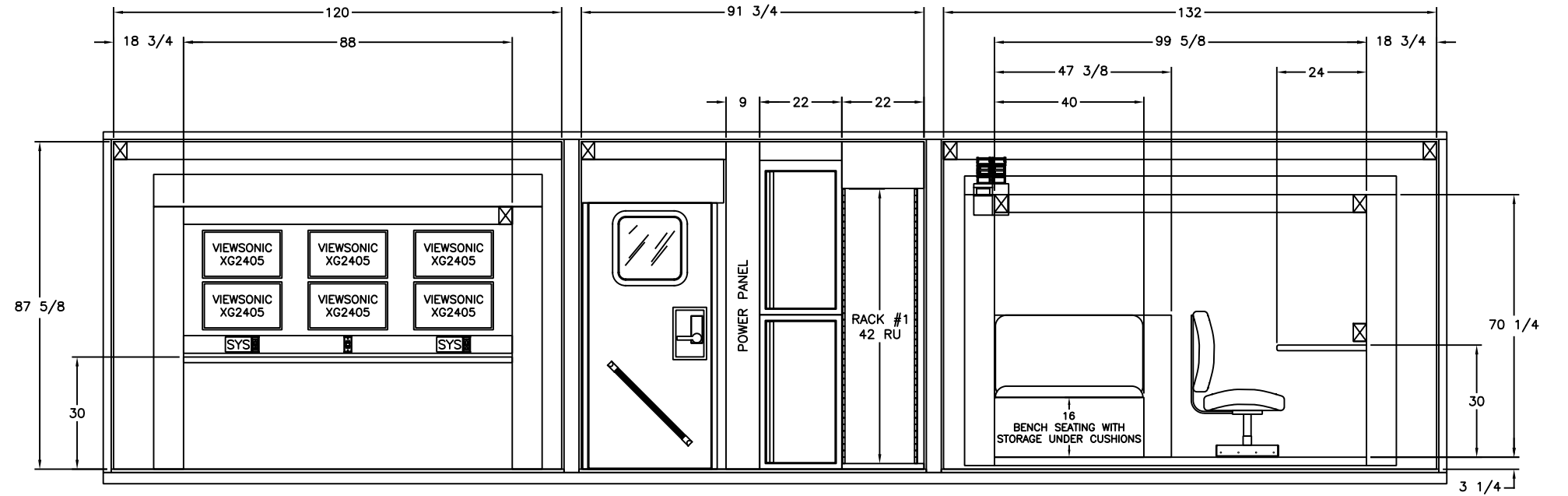
RIGHT SIDE INTERIOR LAYOUT
