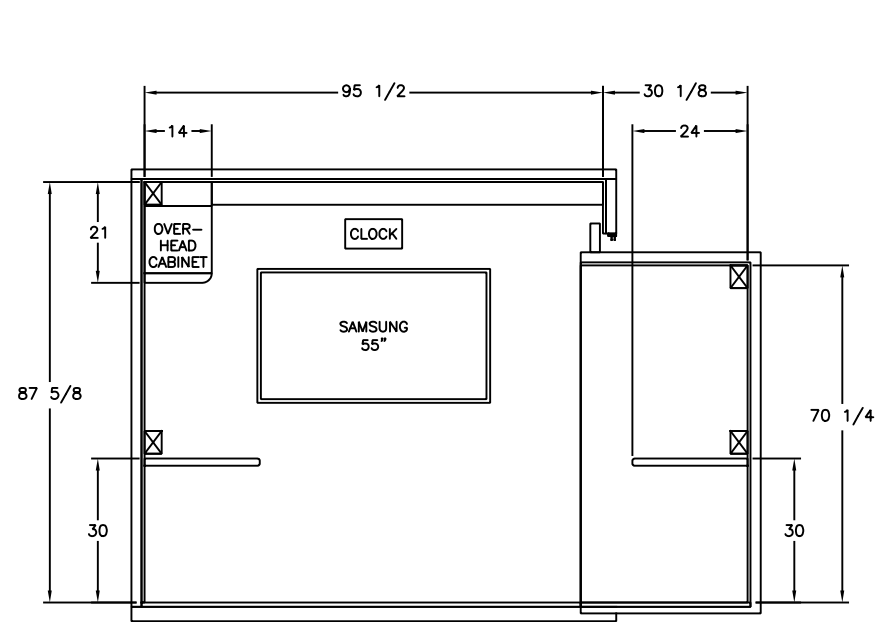
FRONT WALL INTERIOR LAYOUT
