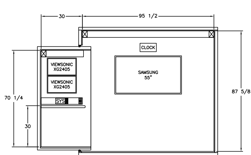
REAR WALL INTERIOR LAYOUT
