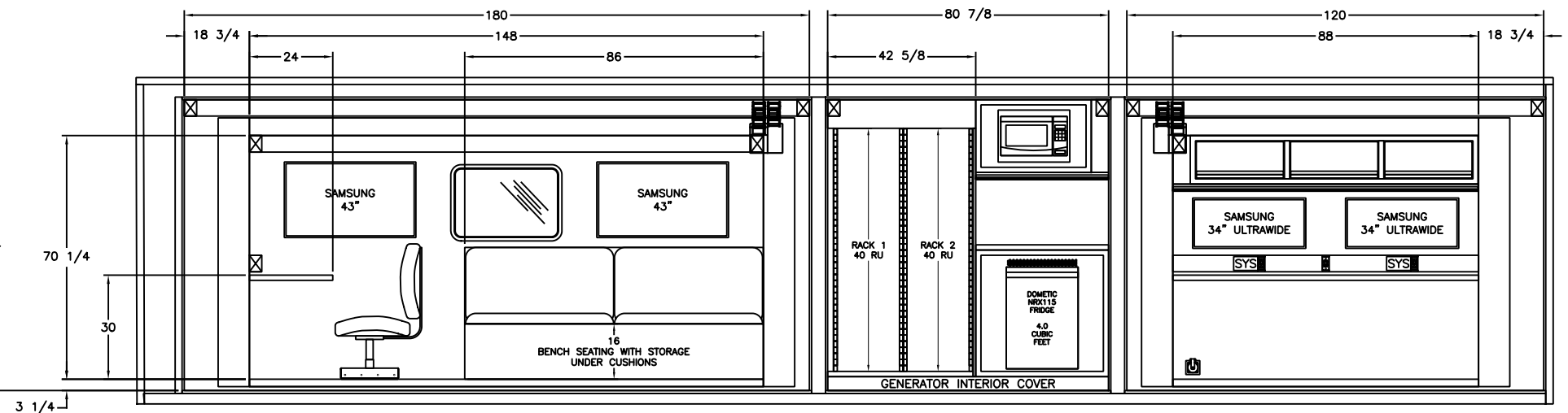
DRIVER SIDE INTERIOR LAYOUT
