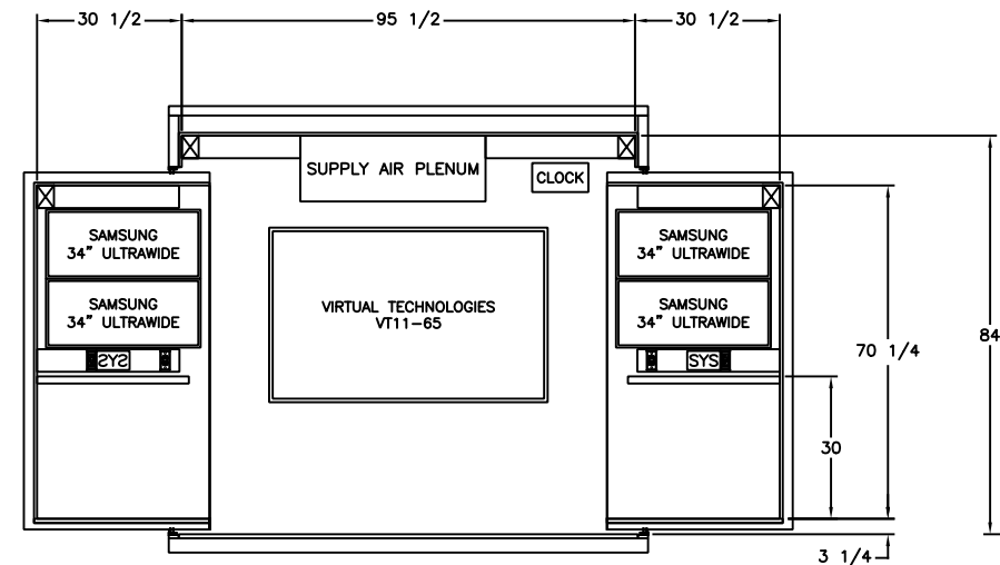
REAR WALL INTERIOR LAYOUT
