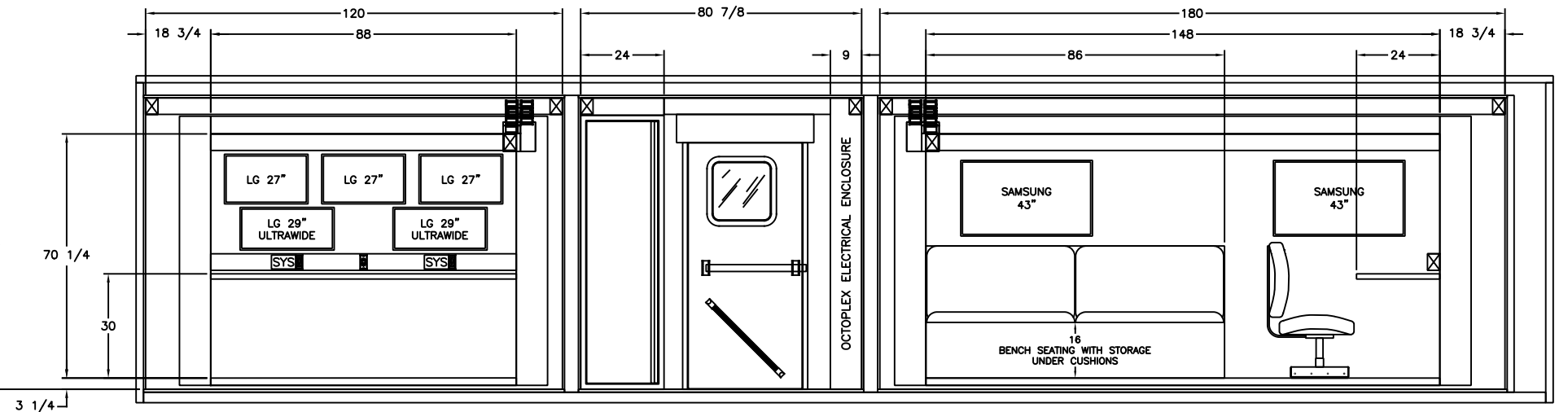
PASSENGER SIDE INTERIOR LAYOUT
