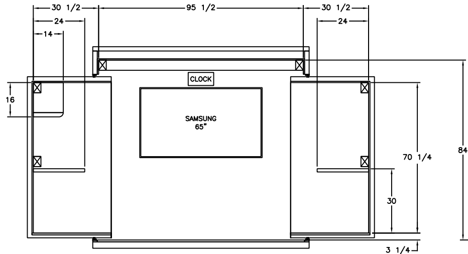
FRONT WALL INTERIOR LAYOUT
