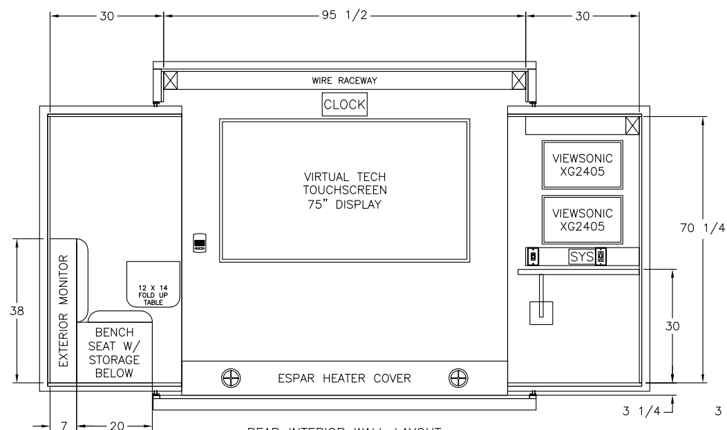
REAR INTERIOR WALL LAYOUT
