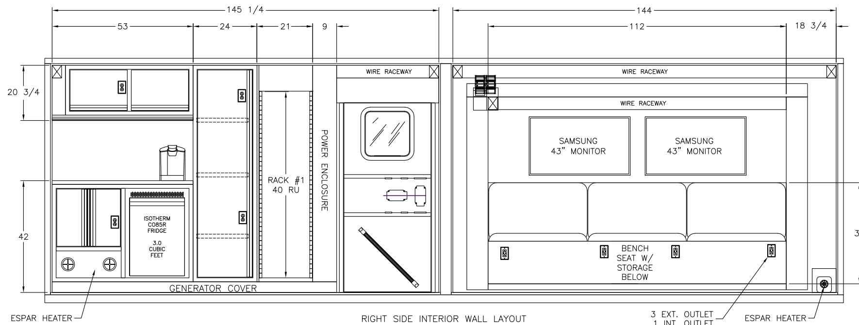
RIGHT SIDE INTERIOR WALL LAYOUT
