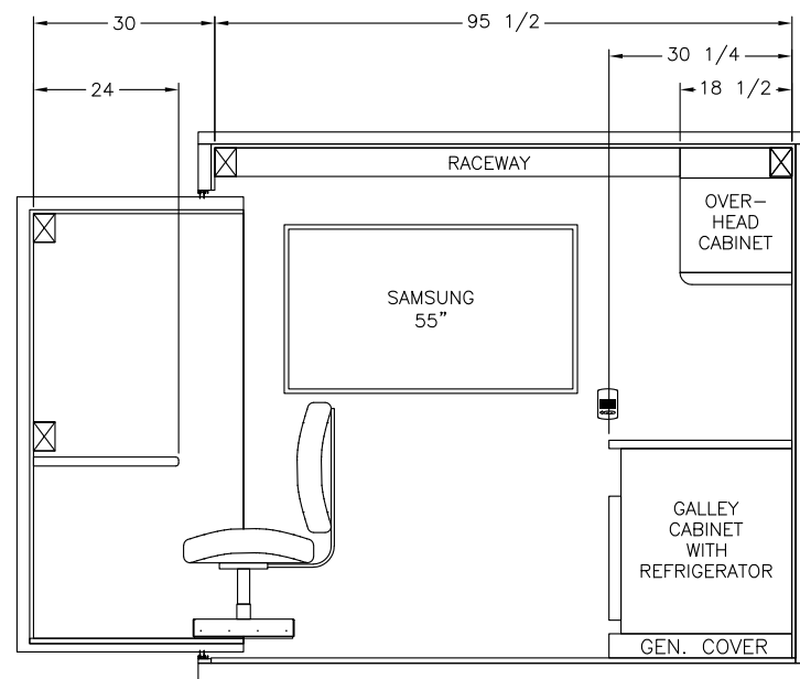
FRONT INTERIOR WALL LAYOUT
