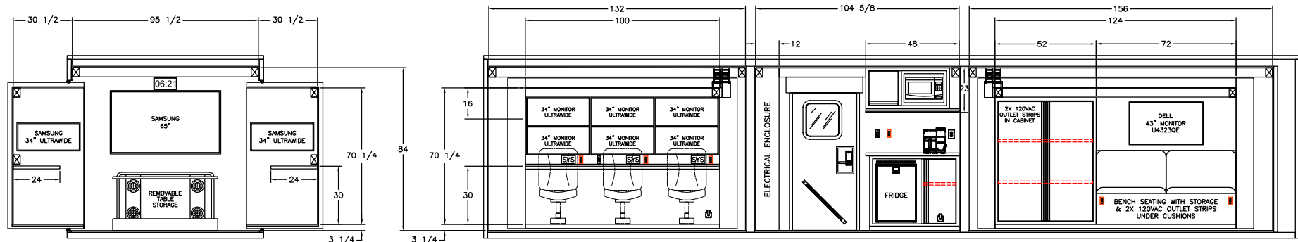
FRONT WALL INTERIOR LAYOUT
