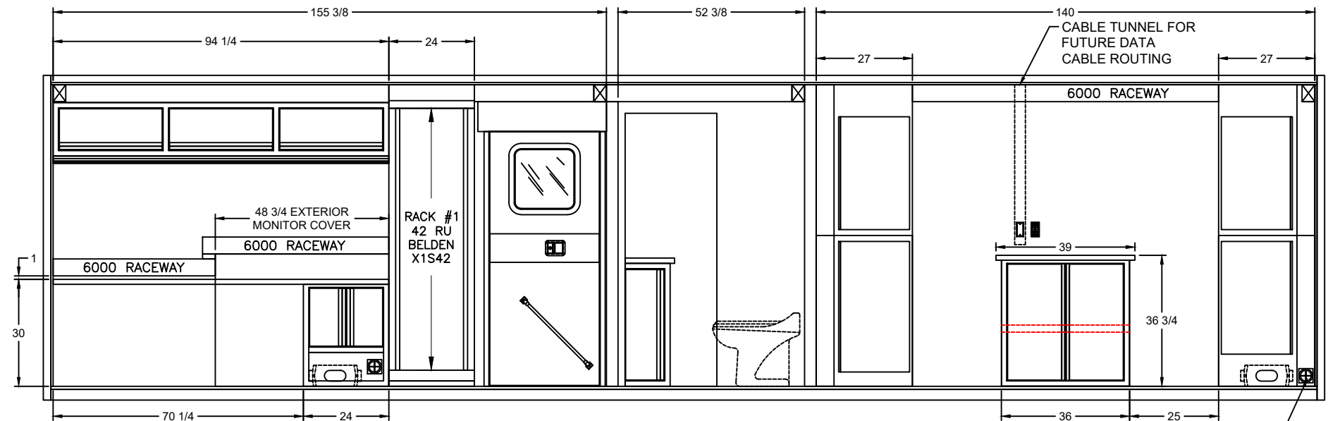
RIGHT SIDE WALL INTERIOR
