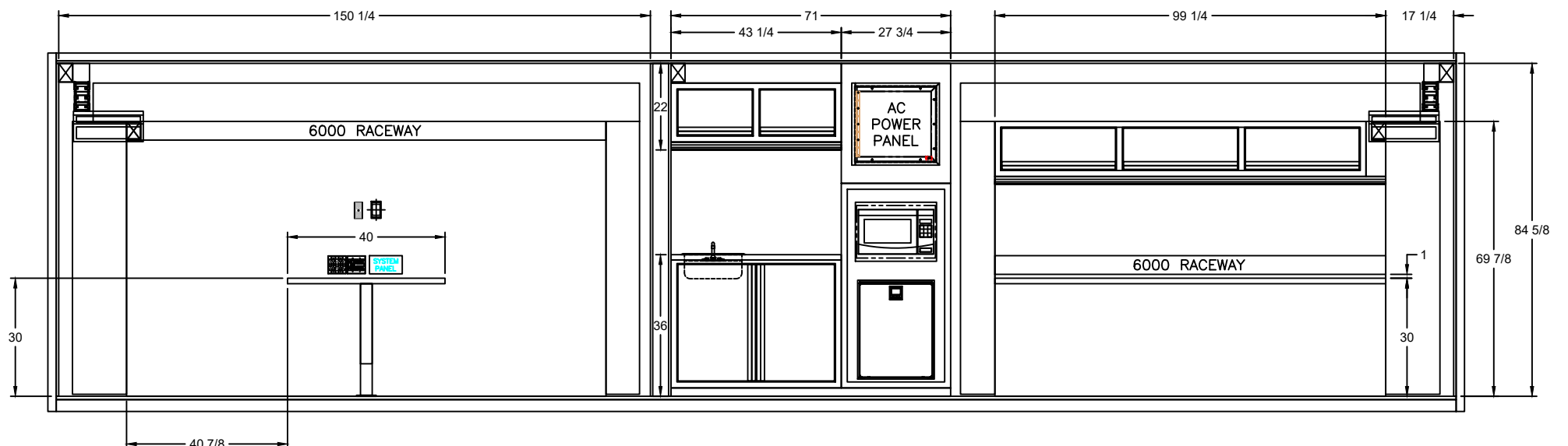
LEFT SIDE WALL INTERIOR
