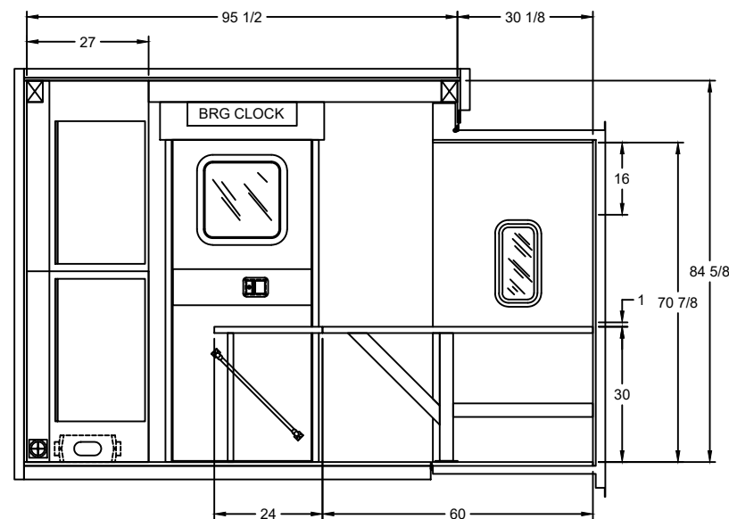
REAR WALL INTERIOR
