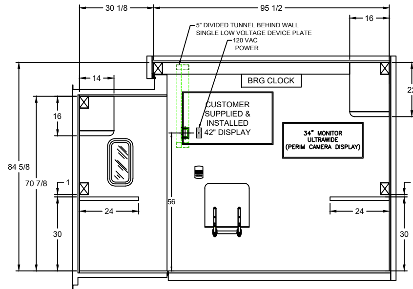
FRONT WALL INTERIOR
